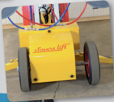
The SL 580 Maxi can be shifted sideways up to 3.9 in for precision adjustment during the window installation process.
